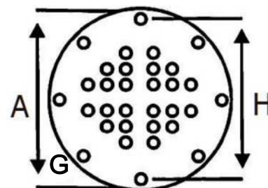
Tubesheet with Bolt Holes
